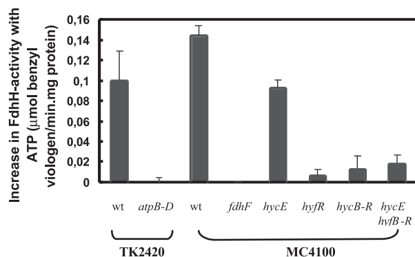
Fig. 2. Increase in Fdh-H activity with ATP in E. coli wild-type, atp , hyc and hyf mutants. The cells were grown and assayed at pH 7.5. The assay mixture contained 0.1 M potassium phosphate pH 7.5. The increase in enzyme activity was the difference between activities in the presence and absence of ATP, 10 mM. Error bars represent the standard deviations from duplicate or triplicate cultures. For wild-type and mutant strains, see Table 1.
